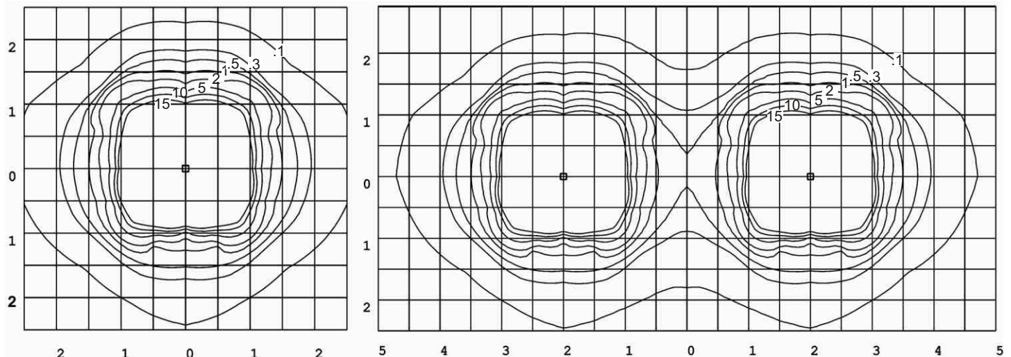
Twin Border Lite G4 20 watt lamp lens height 600mm (24")
