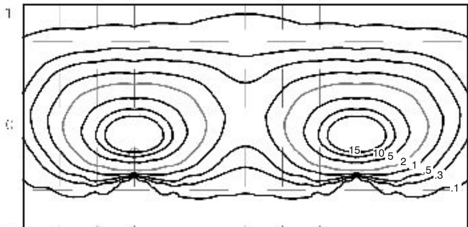
Mouse Lite 10 watt G4 Bi-Pin lamp - Lens height 400mm (15¾")
