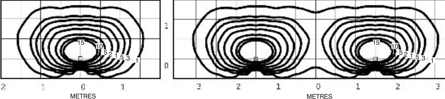
Mouse Lite Square 20 watt GU4 Bi-Pin lamp - Lens height 400mm (15¾")
