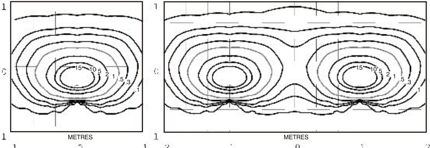
Mouse Lite Square 20 watt GU4 Bi-Pin lamp - Lens height 400mm (15¾")
