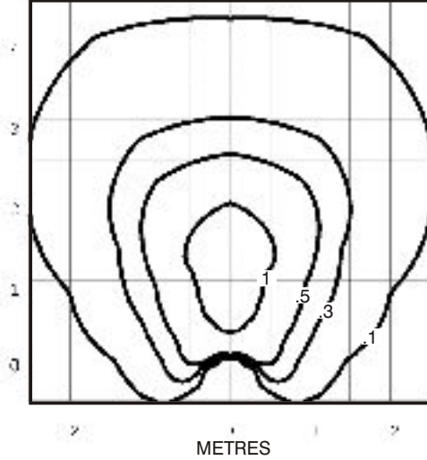
Twig Lite GU4 20 watt Bi-Pin lamp - Lens height 700mm (27½")
